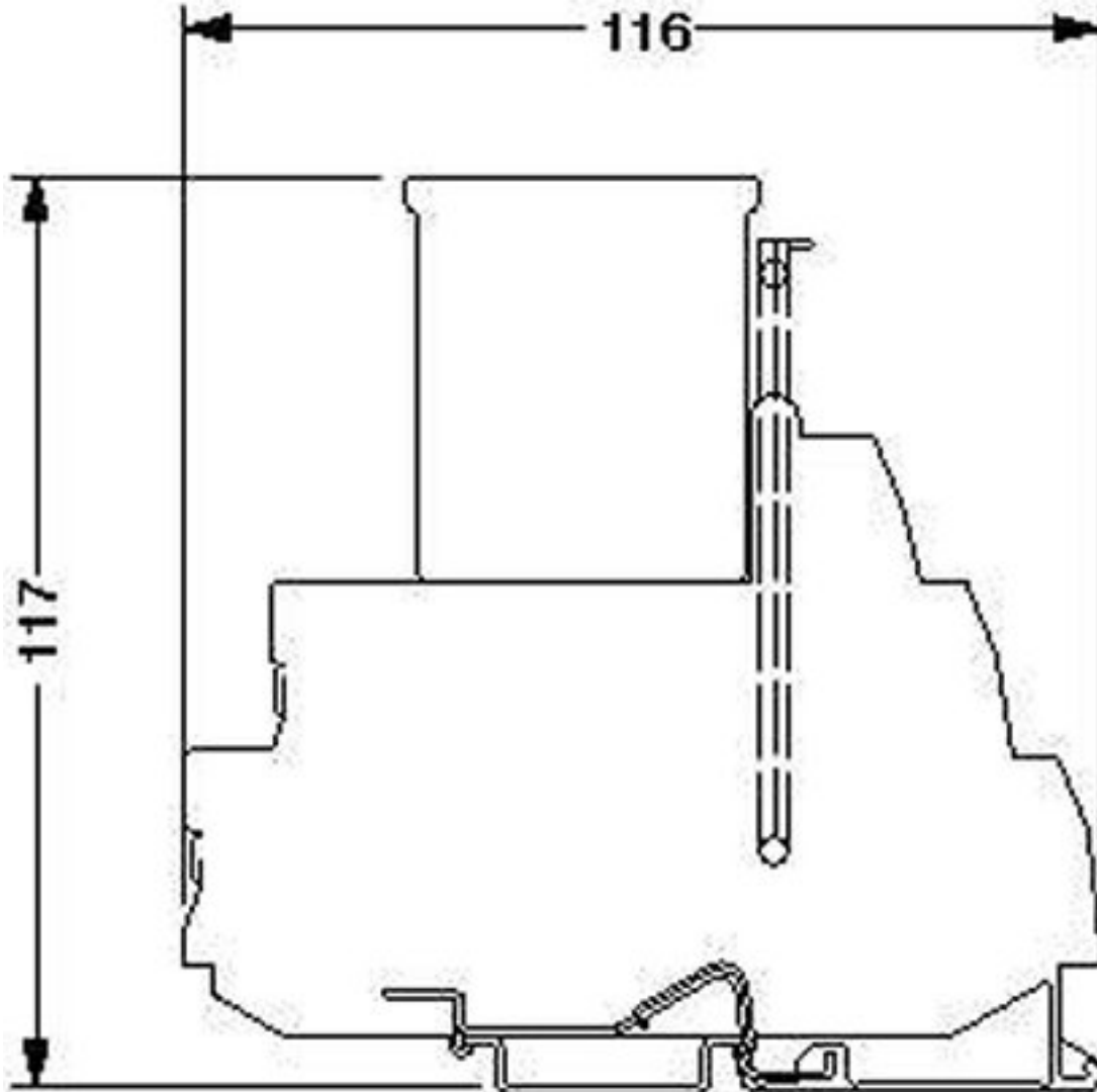
Dimensioned drawing
